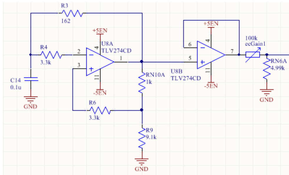
Figure 3.37: Square Wave Oscillator and Gain Stage Reduction Buffer Schematic
