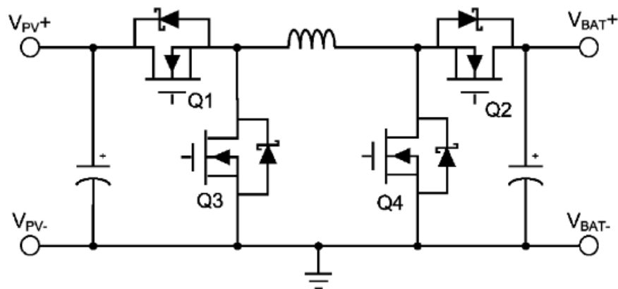
Figure 3.19: DC/DC Converter Stage of Charge Controller [19]. Consent to reproduce figure requested.
