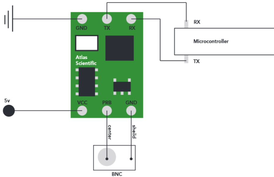
Figure 3.3: Schematic Diagram of the Atlas Scientific EC Meter [11]. Courtesy of Atlas Scientific
