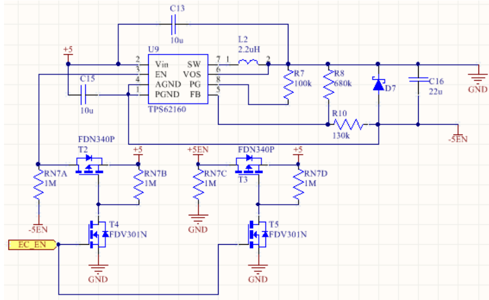
Figure 3.4: Inverting DC/DC Converter and MOSFET Power Switching Schematic
