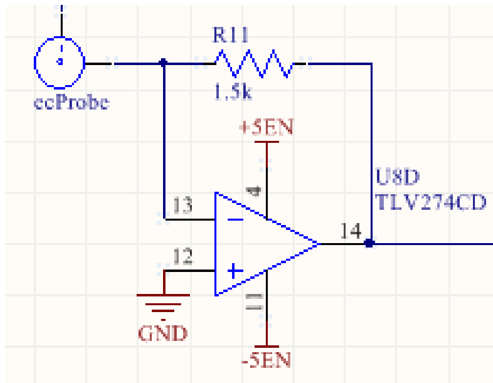
Figure 3.38: Trans-Impedance Amplifier Schematic
