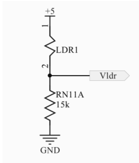
Figure 3.11: Light Sensor Schematic
