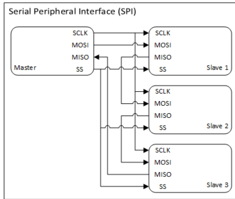
Figure 2.8: SPI Diagram
