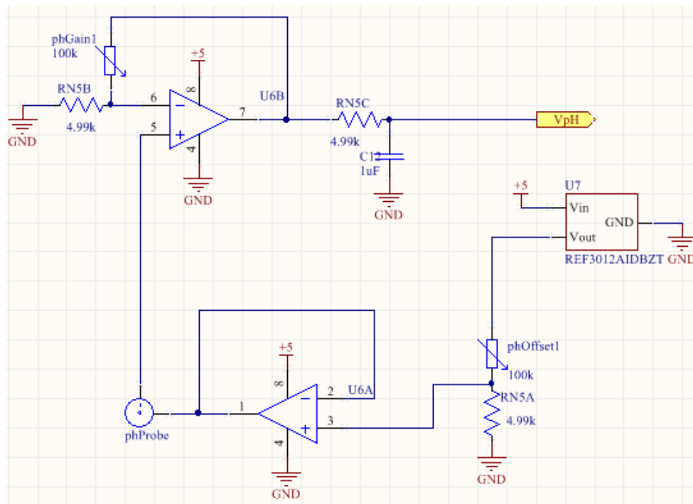
Figure 3.9: pH Interface Schematic
