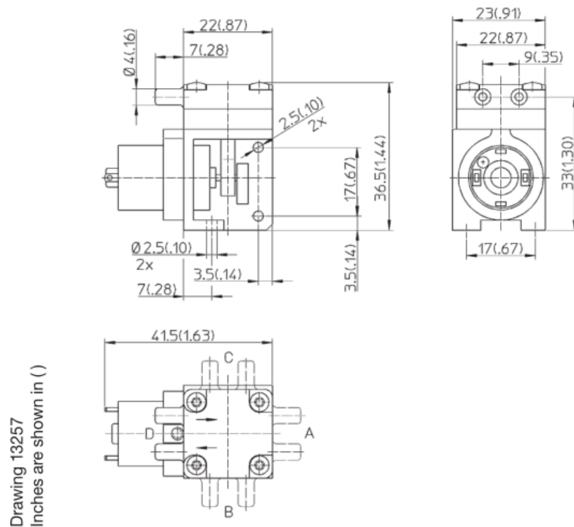
Figure 3.46: Multiview Schematic Drawing of 3003VDLC Diaphragm Pump
