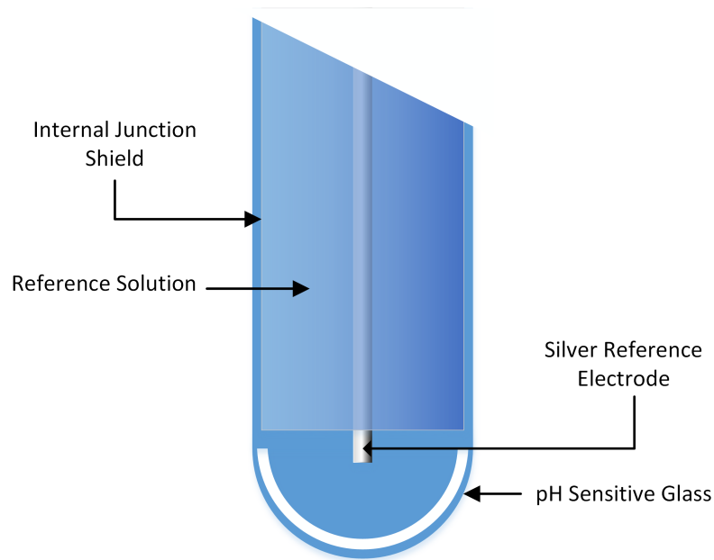
Figure 2.10: Glass Electrode PH Sensor
