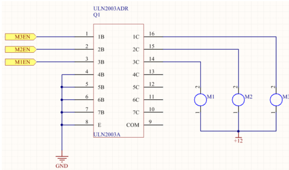
Figure 3.47: Motor Control Schematic
