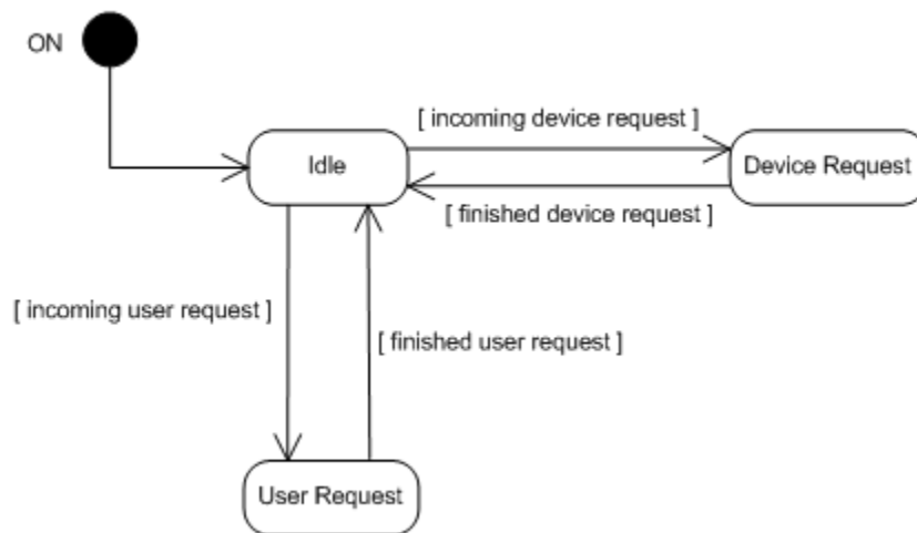
Figure 3.29: Server State Diagram
