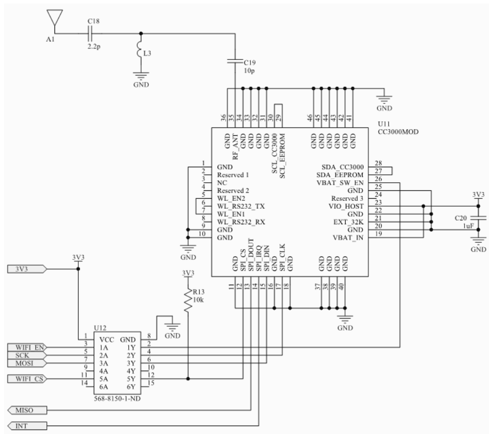
Figure 3.49: CC3000 Wi-Fi Schematic
