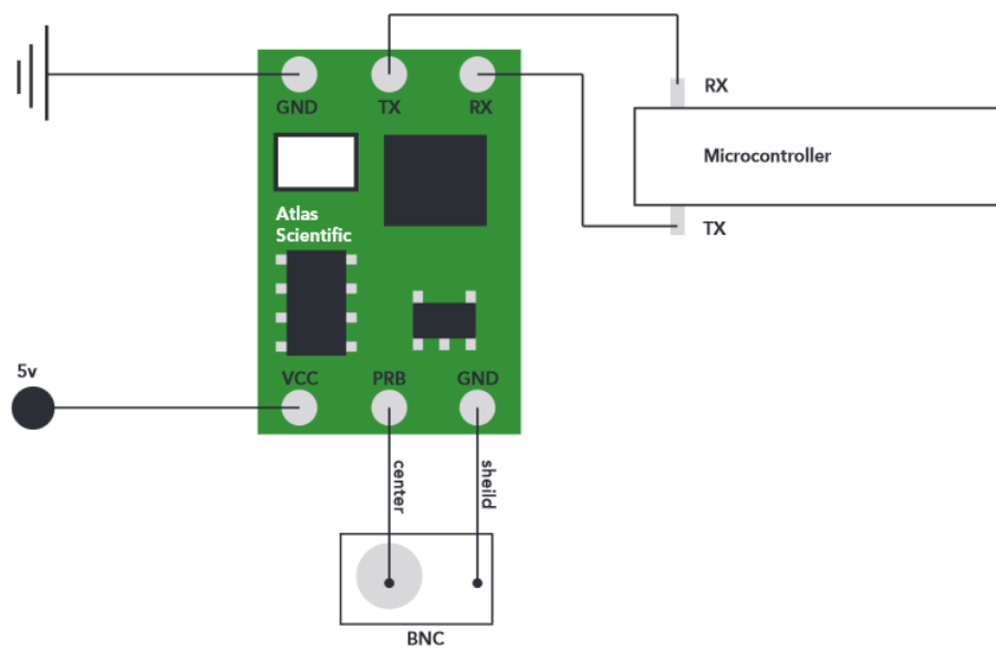
Figure 3.35: Schematic Diagram of the Atlas Scientific EC Meter
