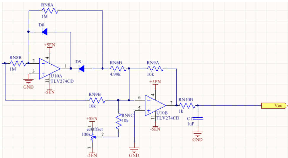
Figure 3.7: Precision Full Wave Rectification and Offset Schematic
