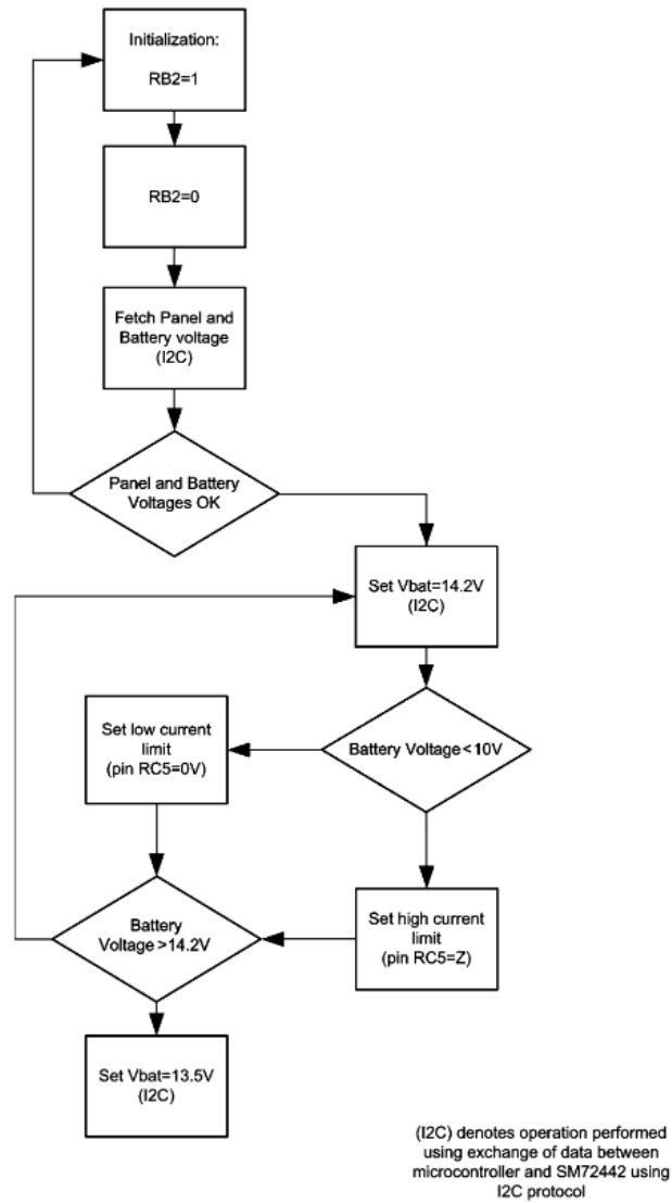
Figure 3.21: Operational Flow Chart for Charge Controller [19]. Consent to reproduce figure requested.
