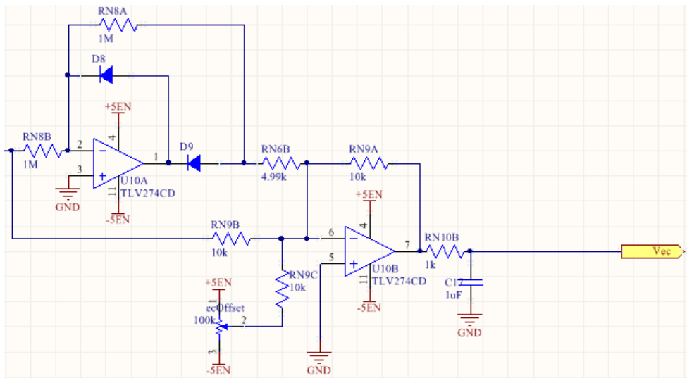
Figure 3.39: Precision Rectifier Schematic
