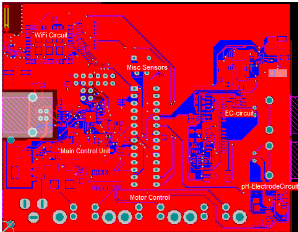
Figure 4.1: PCB Gerber Layout
