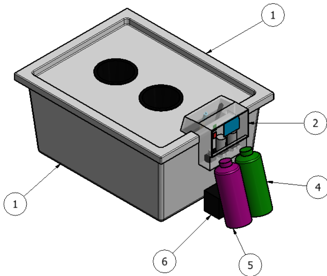
Figure 3.54: Overall Placement of Parts in Hydroponics System
