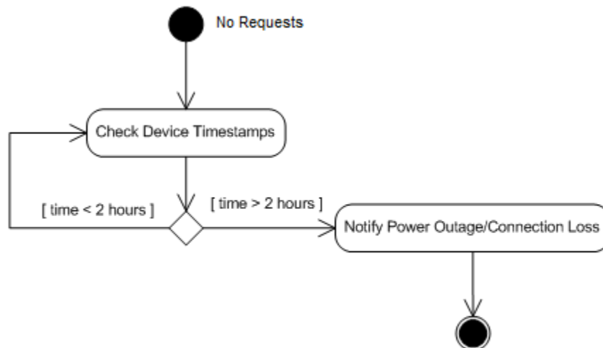
Figure 3.28: Server Activity Diagram (Idle)
