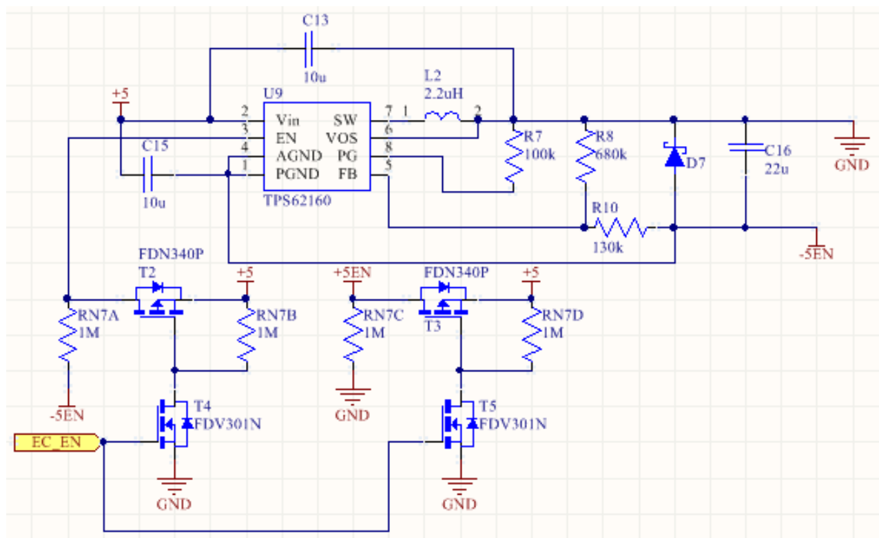
Figure 3.36: Inverting DC/DC Converter and MOSFET Power Switching Schematic
