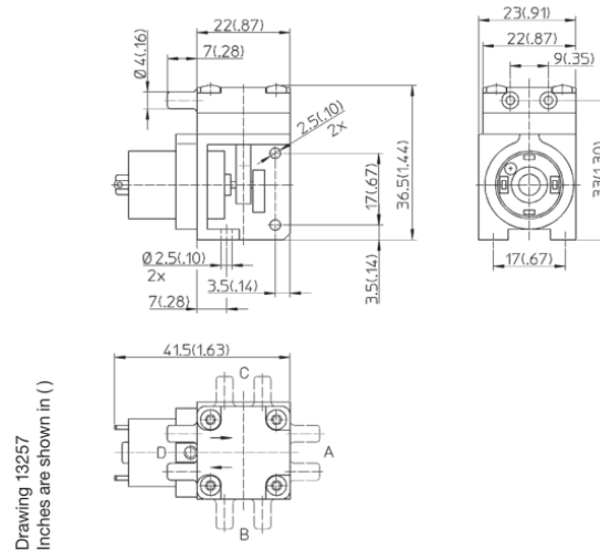
Figure 3.14: Multiview Schematic Drawing of 3003VDLC Diaphragm Pump [6]. Consent to reproduce figure requested.
