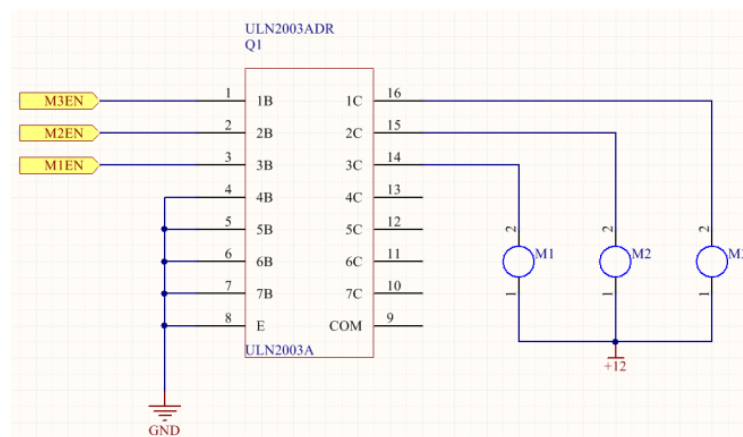
Figure 3.15: Motor Control Schematic
