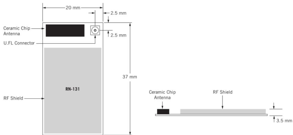
Figure 3.48: A Multiview Schematic Drawing of the RN131G Wi-Fi Transceiver
