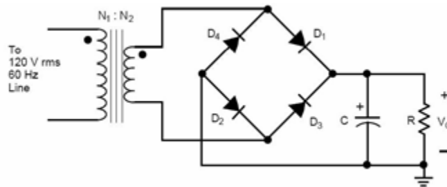
Figure 2.9: Full Wave Rectifier Circuit Diagram
