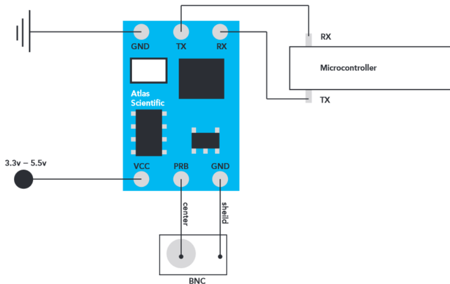
Figure 3.8: Schematic Diagram of the Atlas Scientific pH Meter [17]. Courtesy of Atlas Scientific
