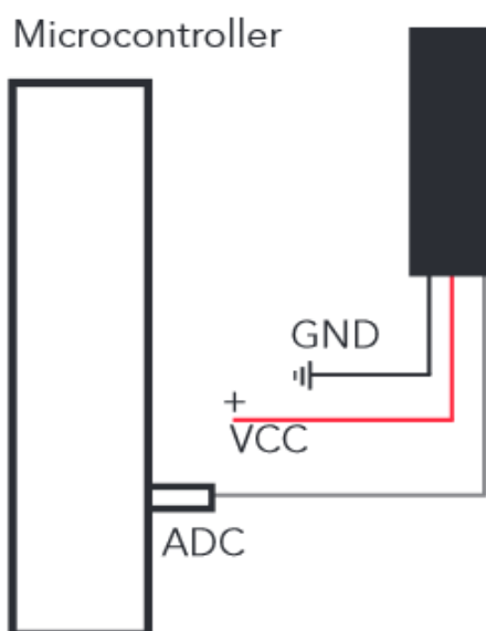
Figure 3.42: Schematic Diagram of the Atlas Scientific Temperature Meter
