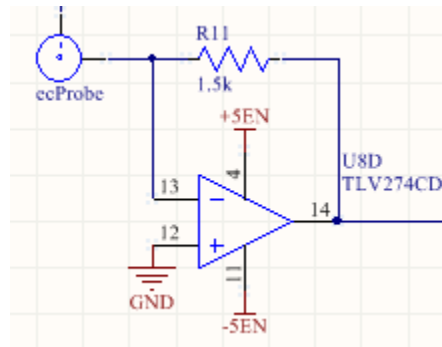
Figure 3.6: Trans-Impedance Amplifier Schematic
