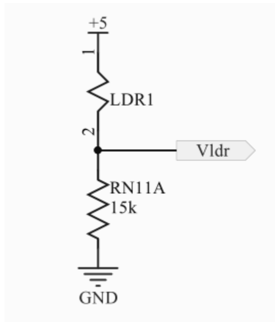
Figure 3.43: Light Sensor Schematic
