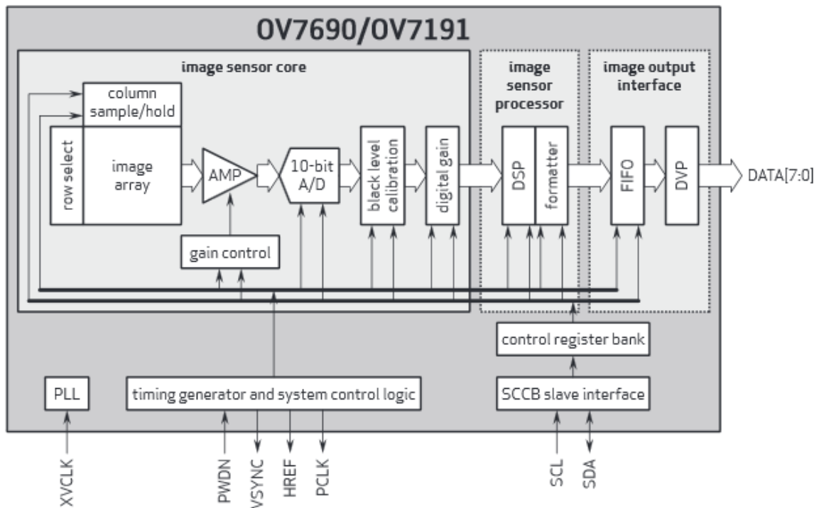
Figure 2.12: Functional Block Diagram for OV7960 [14]. Consent to reproduce figure requested
