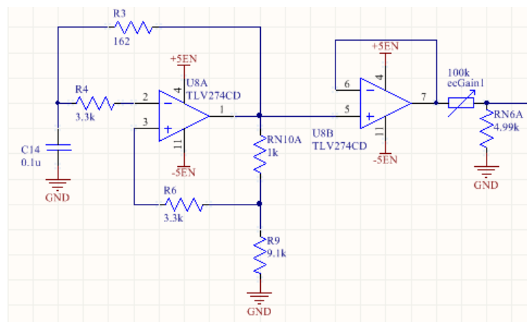
Figure 3.5: Square Wave Oscillator and Gain Stage Reduction Buffer Schematic
