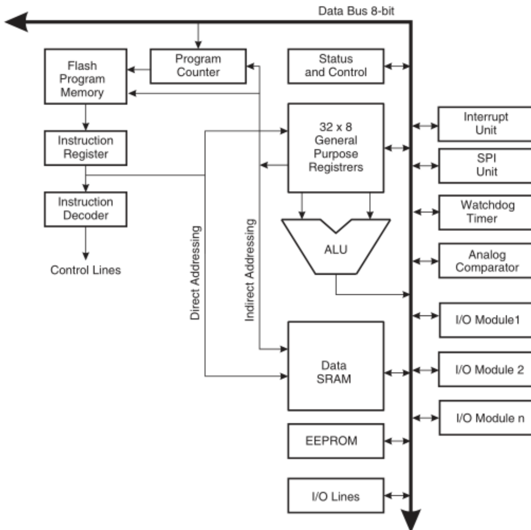
Figure 3.23: Microprocessor Block Diagram [7]. Courtesy of Atmel
