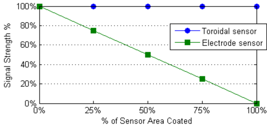
Figure 2.11: Deterioration of Electrode vs Toroidal Sensors
