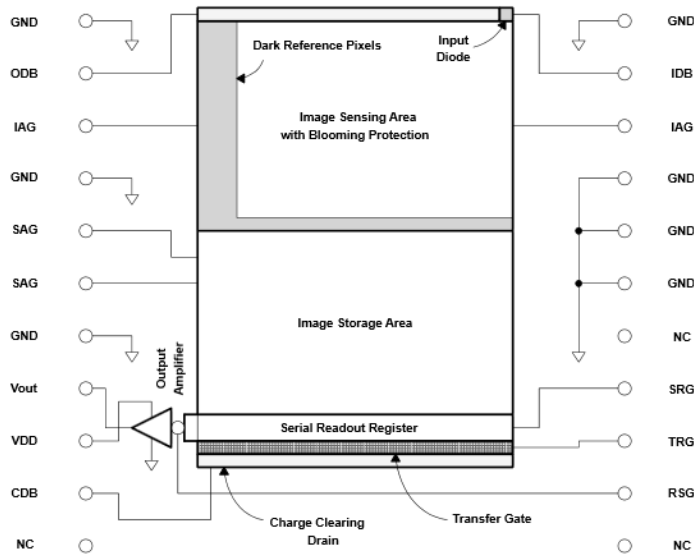
Figure 2.13: Texas Instruments TC341 Image Sensor Diagram [21]. Courtesy of Texas Instruments
