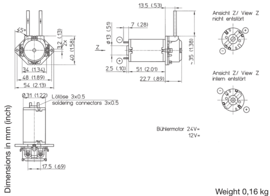
Figure 3.45: Multiview Schematic Drawing of SR10/30 DC Straight Flange Pump
