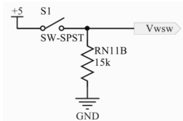
Figure 3.12: Water Switch Schematic
