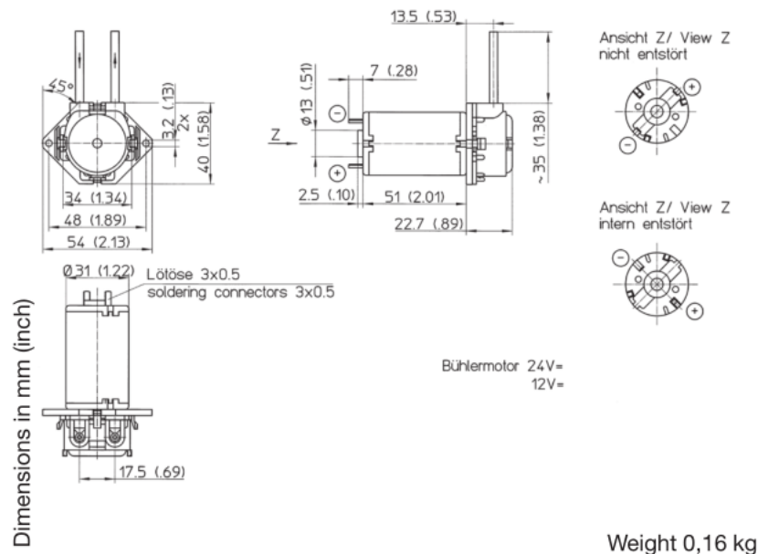
Figure 3.13: Multiview Schematic Drawing of SR10/30 DC Straight Flange Pump [20]. Consent to reproduce figure requested
