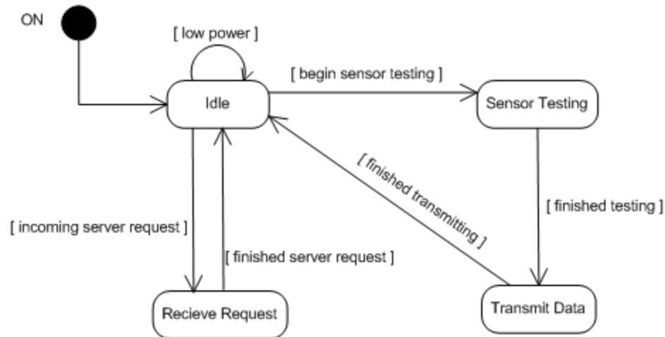
Figure 3.26: System State Diagram
