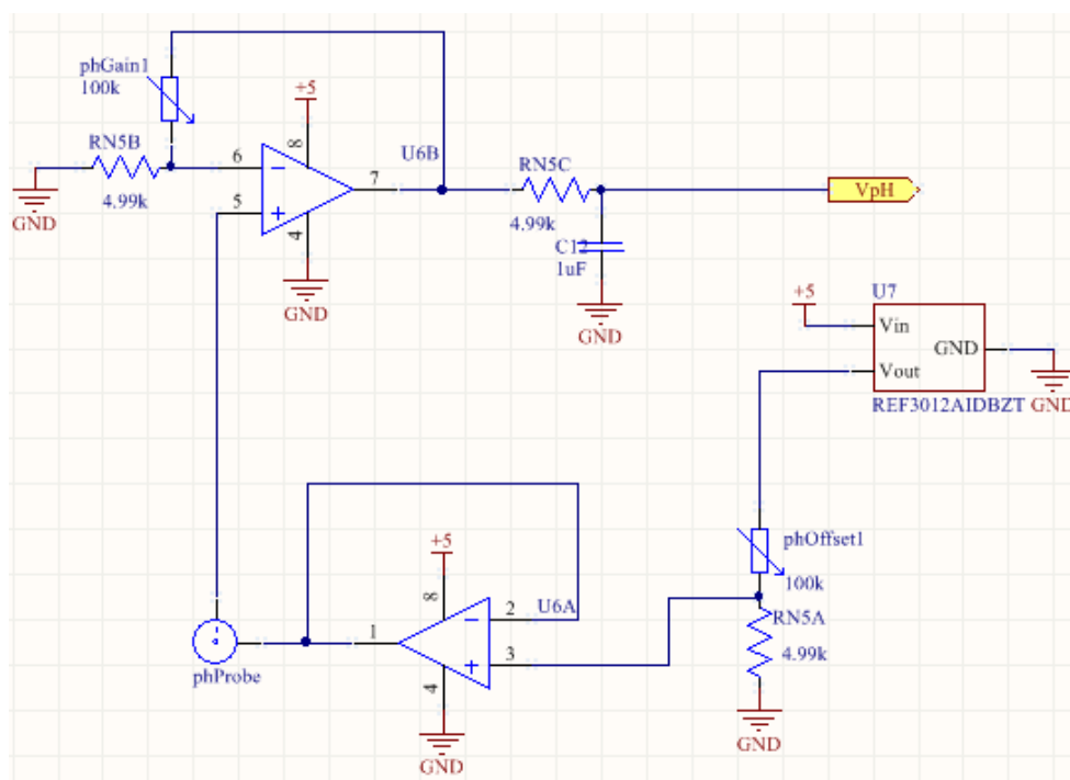
Figure 3.41: pH Interface Schematic
