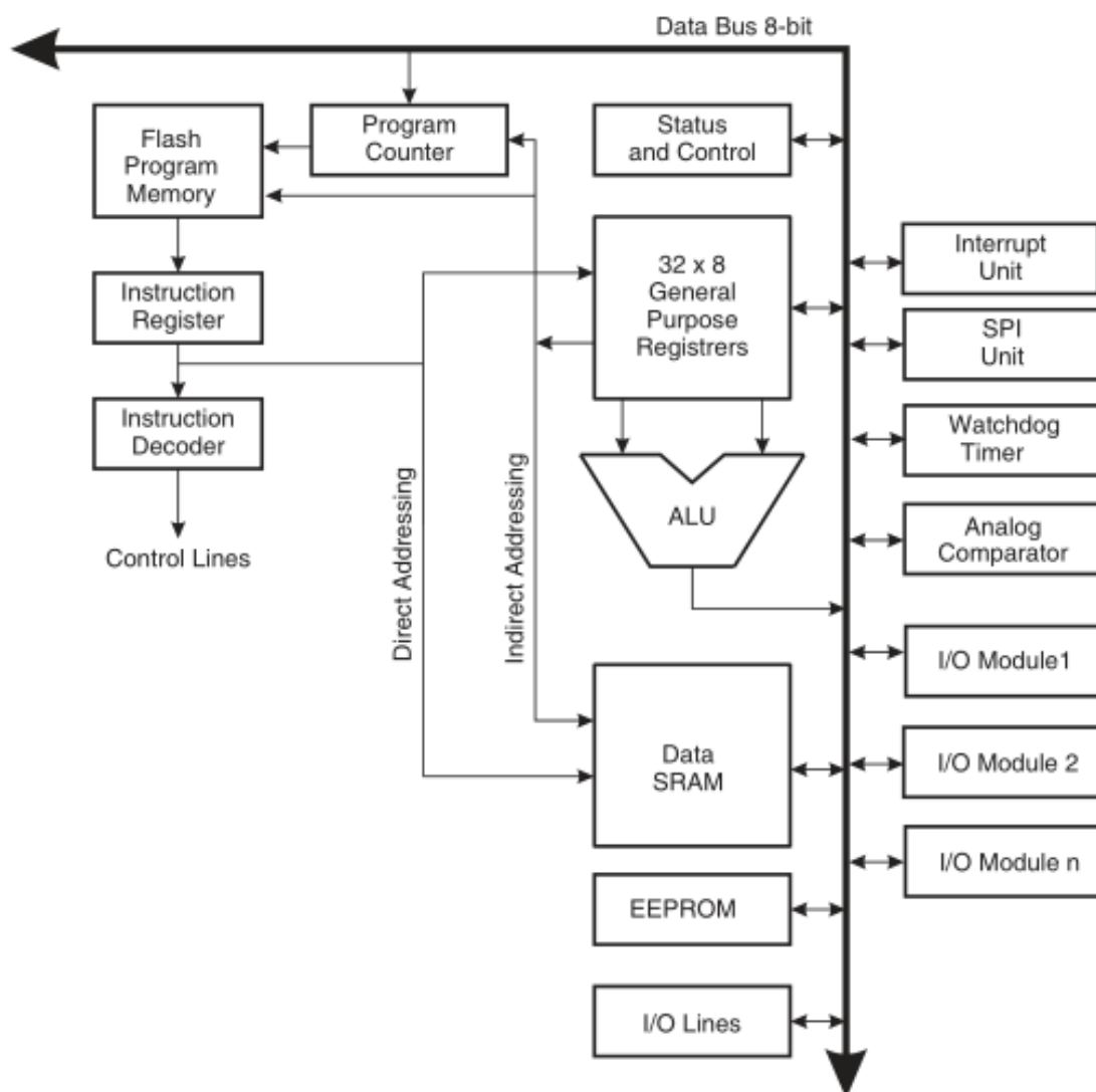
Figure 3.50: Microprocessor Block Diagram
