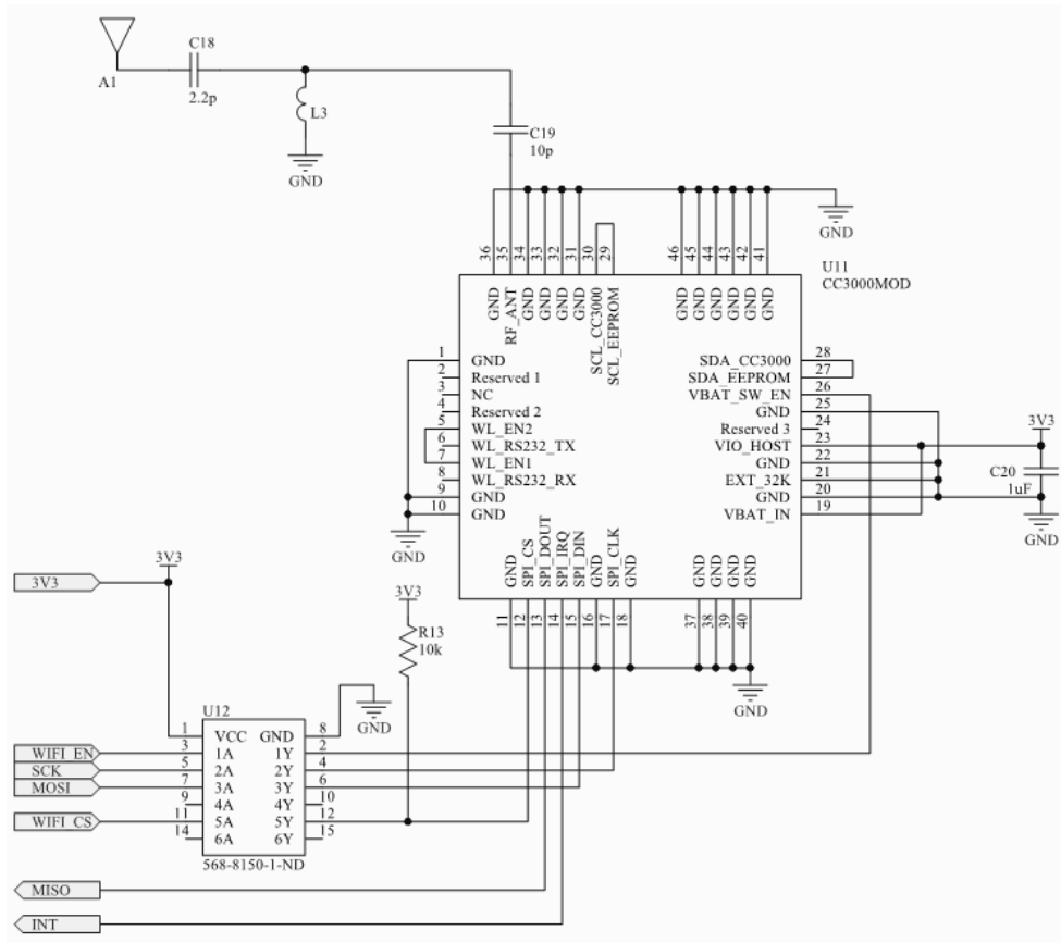
Figure 3.22: CC3000 Wi-Fi Schematic
