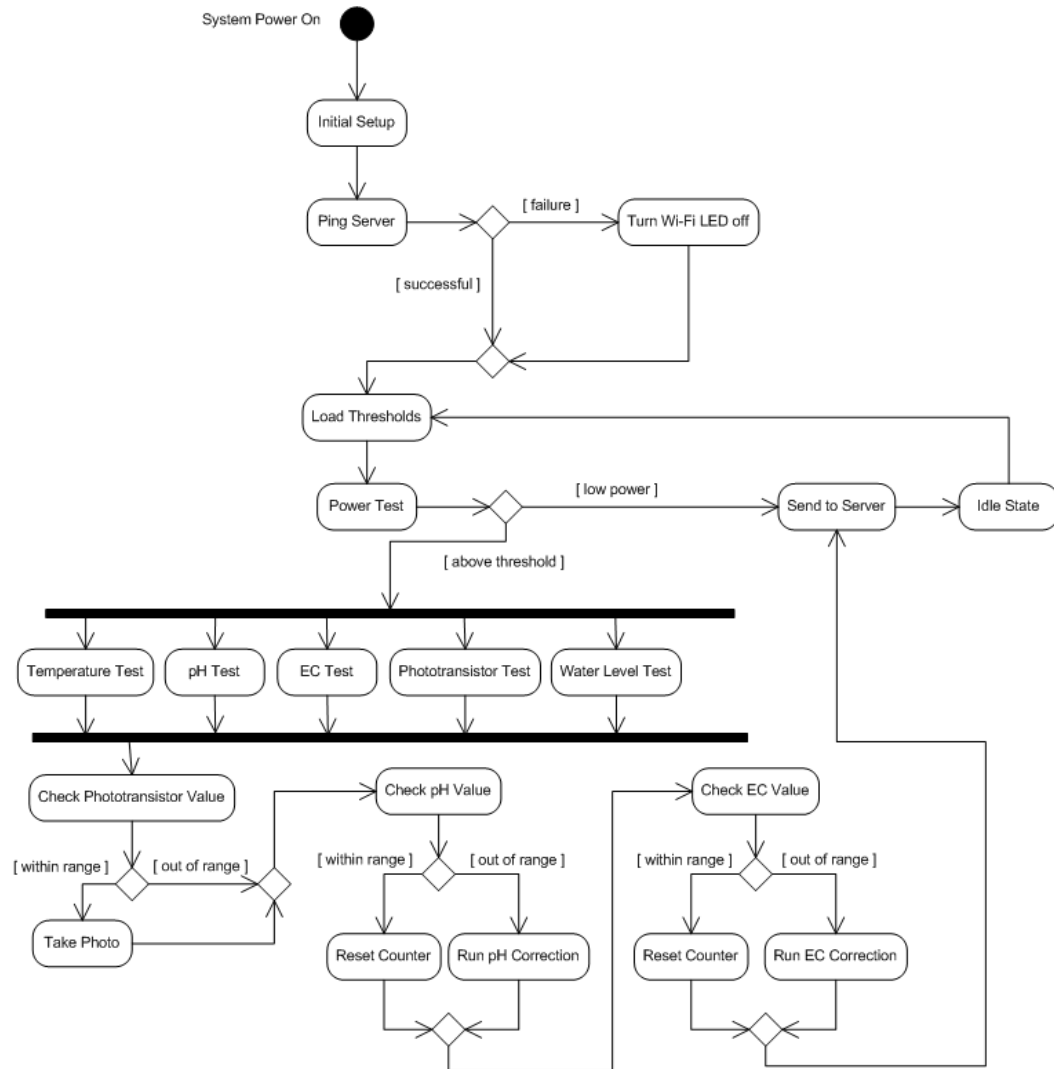
Figure 3.25: System Activity Diagram
