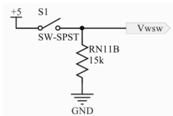
Figure 3.44: Water Switch Schematic
