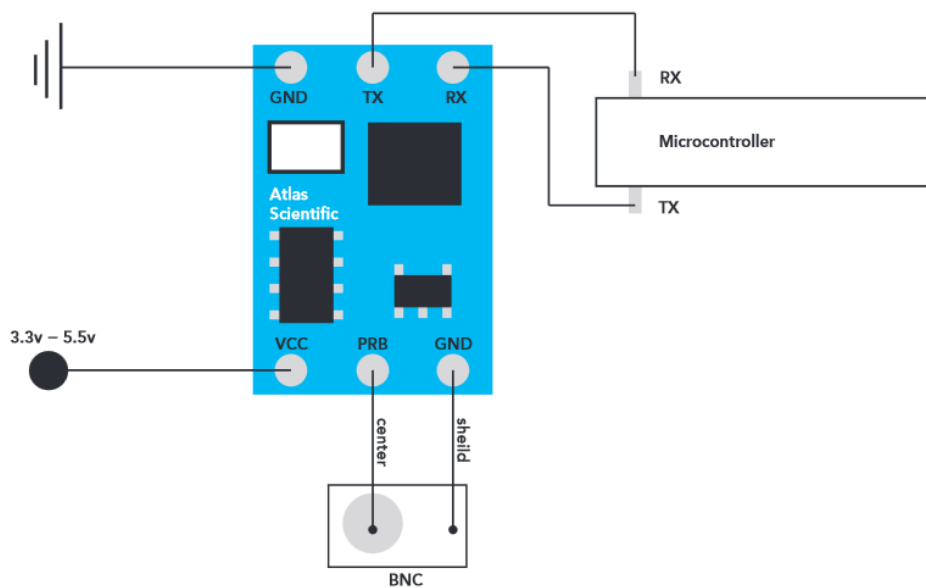
Figure 3.40: Schematic Diagram of the Atlas Scientific pH Meter
